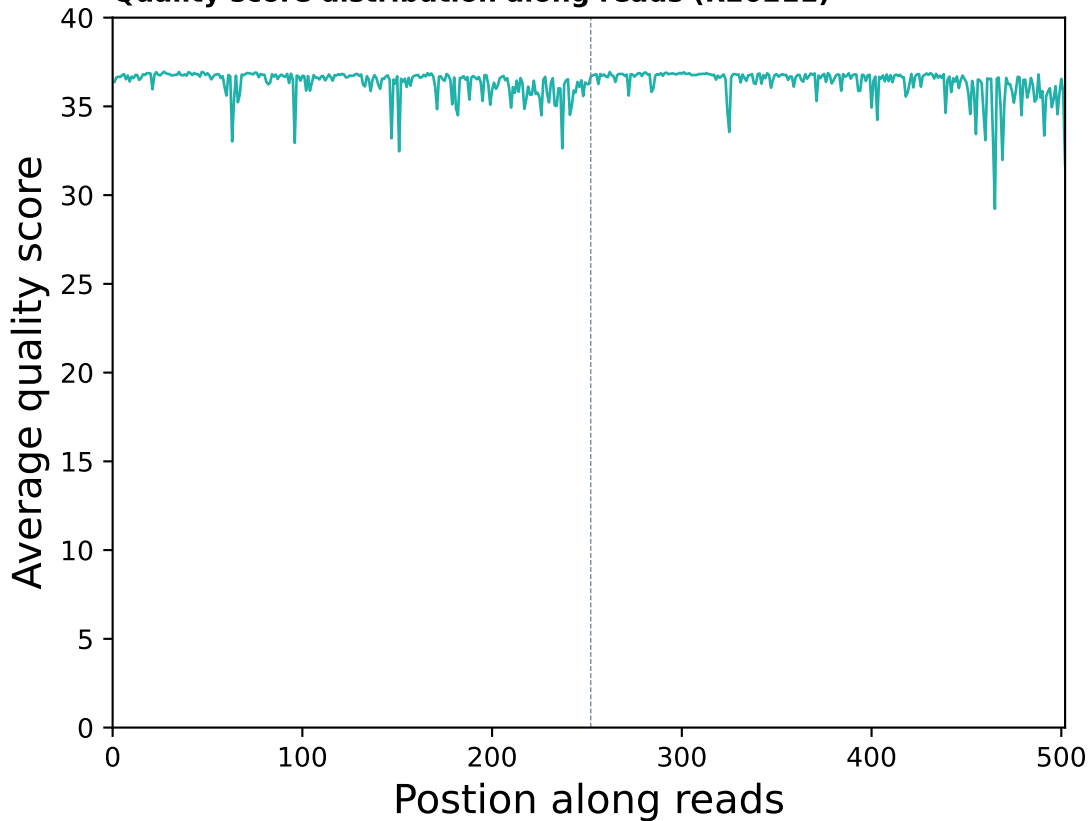
Quality score distribution along reads (R20211)
